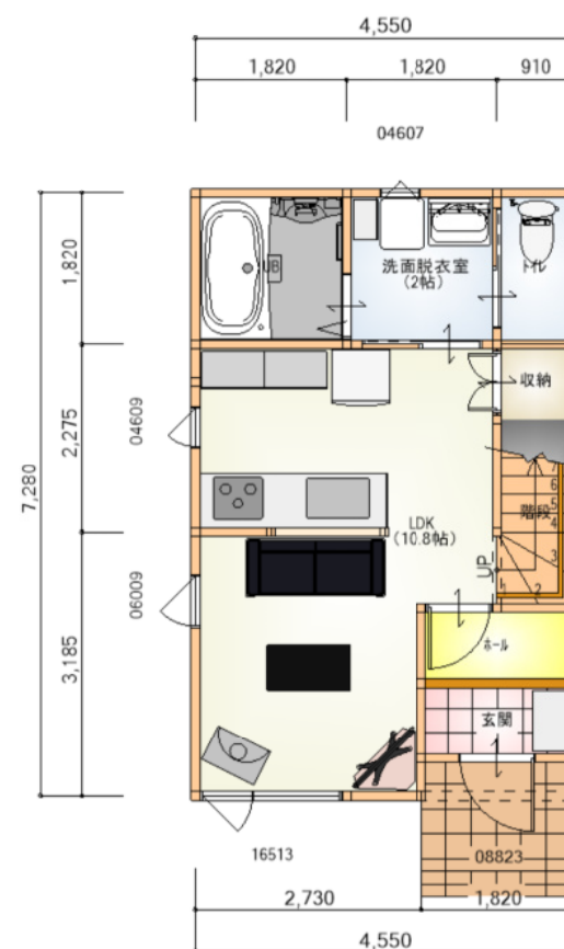
1st FLOOR
