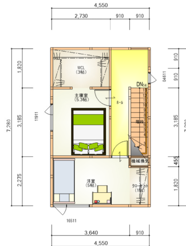
2nd FLOOR
