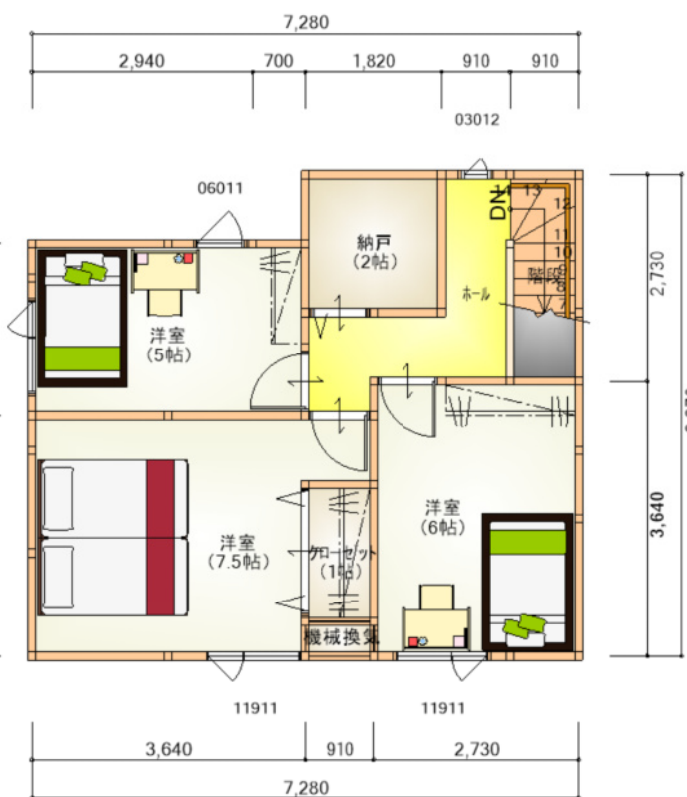
2nd FLOOR
