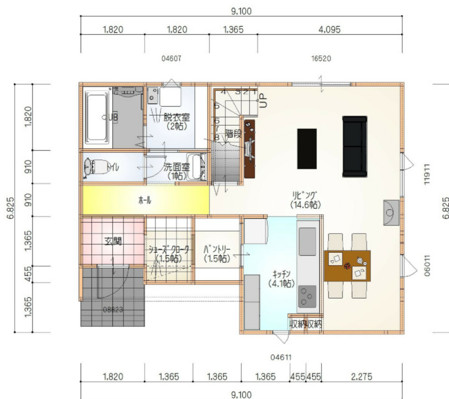
1st FLOOR
