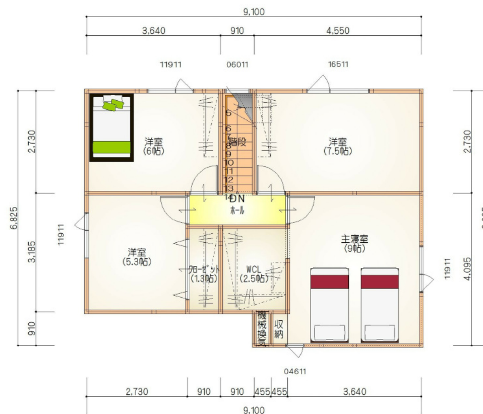
2nd FLOOR
