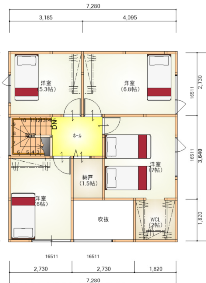
2nd FLOOR
